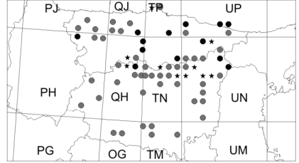
Hesperia comma
