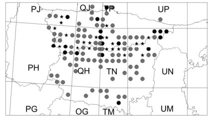
Carcharodus alceae
