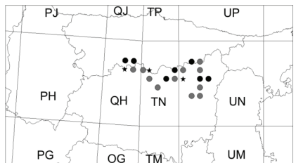
Pyrgus carthami
